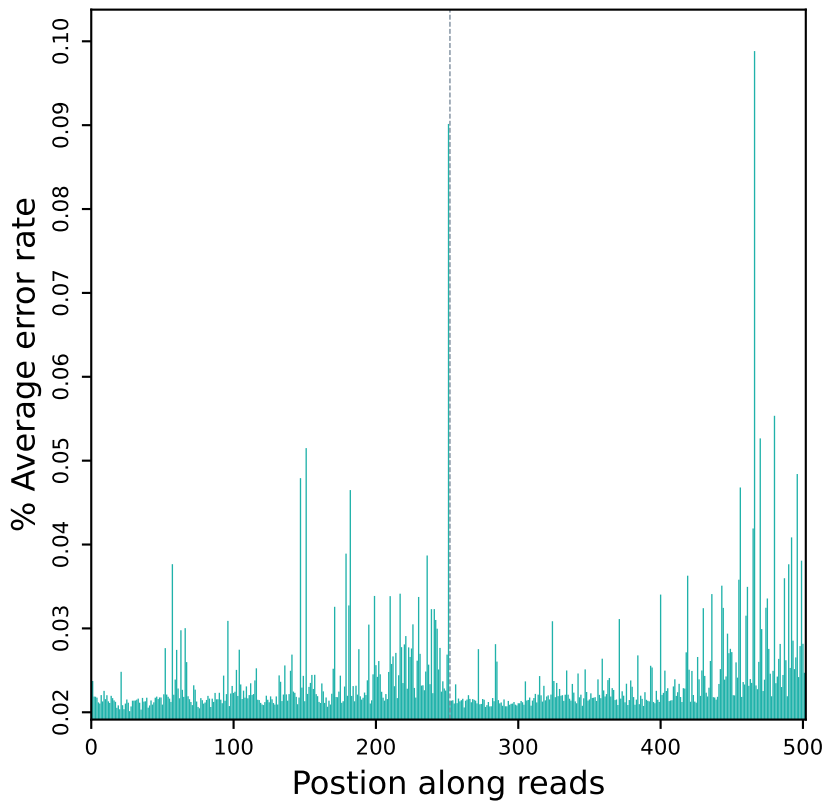
Error rate distribution along reads (R10413)
